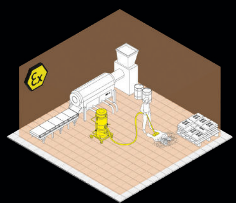
Combustible or non-combustible dust inside an ATEX Zone 22: accessories and vacuum cleaner inside an ATEX area.
