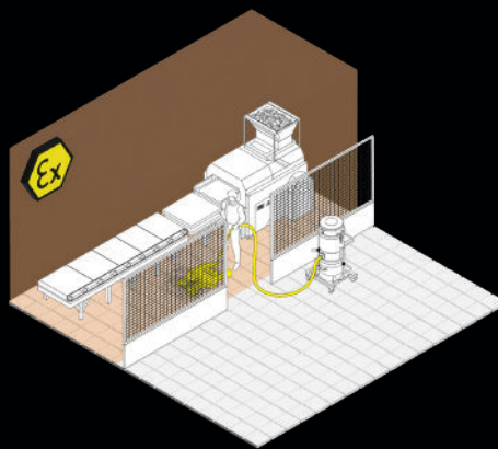
Combustible dust within an ATEX Zone 22: accessories inside, vacuum cleaner outside an ATEX area.
