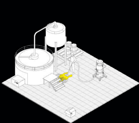
Combustible dust outside of an ATEX Zone 22: accessories and vacuum cleaner in a non-ATEX area.
